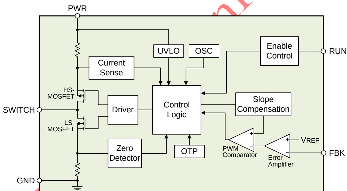
Figure 1. EA8103A internal function block diagram
