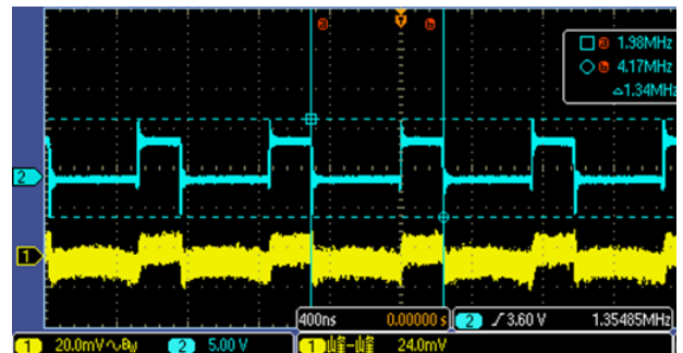
VIN = 5V, ILOAD = 1.2A Waveform
