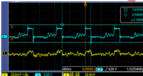
VIN = 5V, ILOAD = 0.1A Waveform
