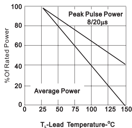
FIG. 2-Power Derating Curve
