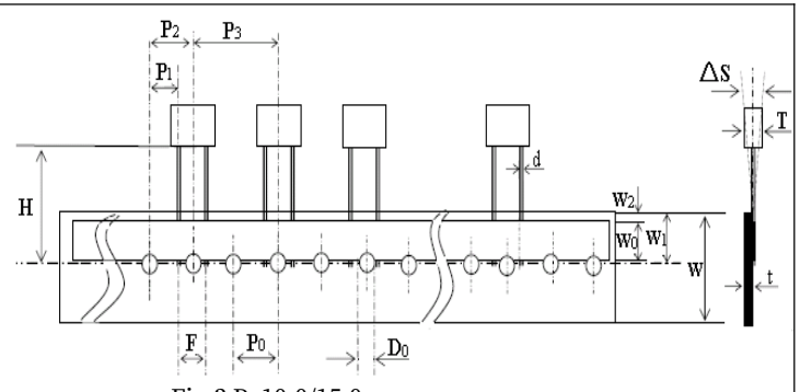
Fig.2 P=10.0/15.0mm
