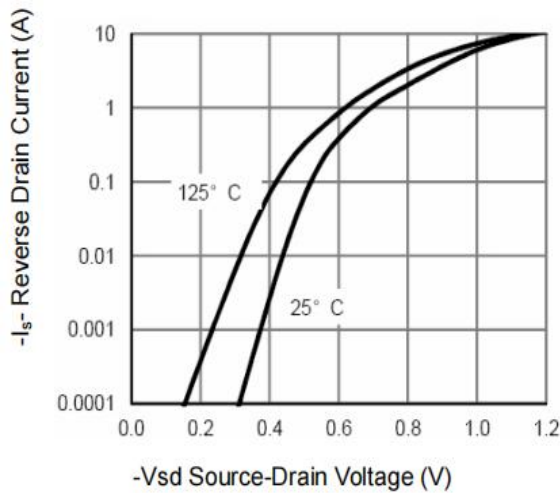
Figure 9: Diode Characteristics
