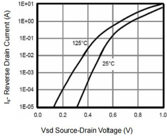
Figure 7: Diode Characteristics
