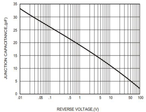
Figure 4: Junction Capacitance
