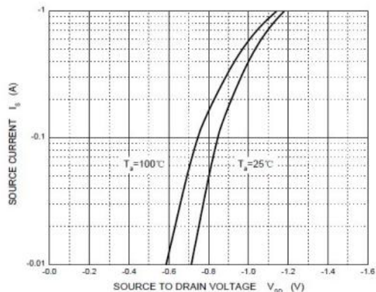
Figure 5: Diode Characteristics
