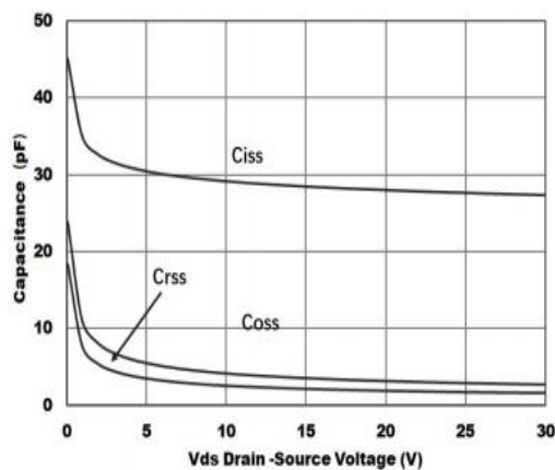
Figure 4: Capacitance Characteristics
