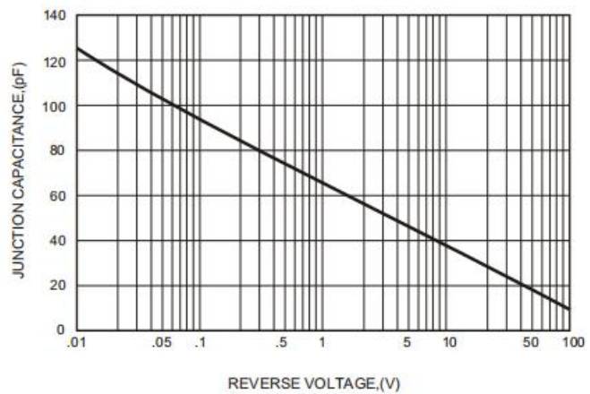
FIG.5-TYPICAL JUNCTION CAPACITANCE
