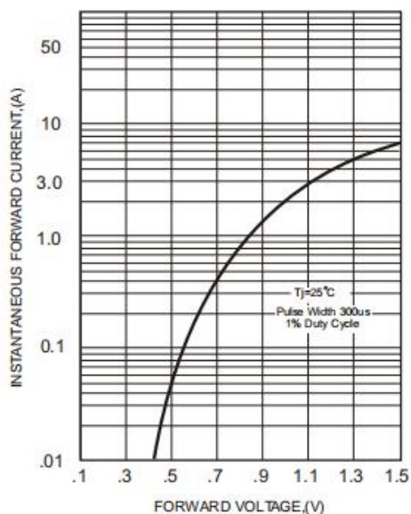
FIG.2-TYPICAL FORWARD CHARACTERISTICS
