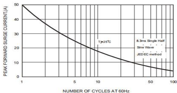
Figure 2: Peak Forward Surge Current
