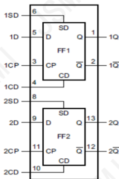
Figure 1. Functional diagram
