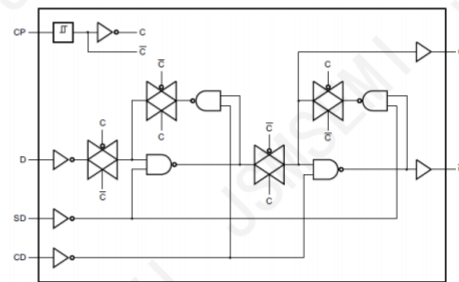
Figure 2. Logic diagram (one flip-flop)
