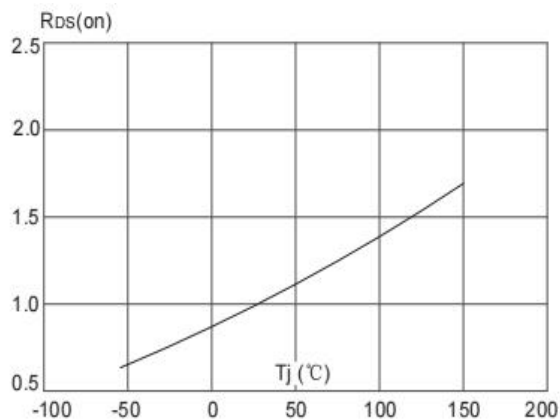
Figure 7: On-Resistance vs. T_j
