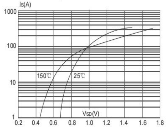
Figure 2: Diode Forward Characteristics
