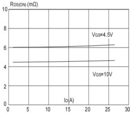
Figure 3: On-Resistance vs. I_D
