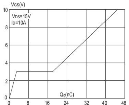
Figure 6: Gate-Charge Characteristics
