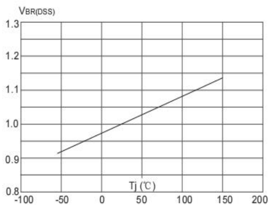
Figure 8: Breakdown Voltage vs. T_j
