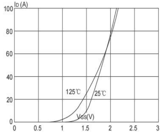
Figure 4: Transfer Characteristics
