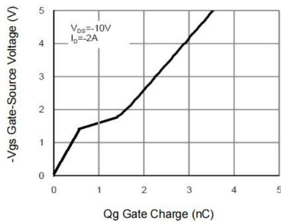
Figure 6: Gate-Charge Characteristics
