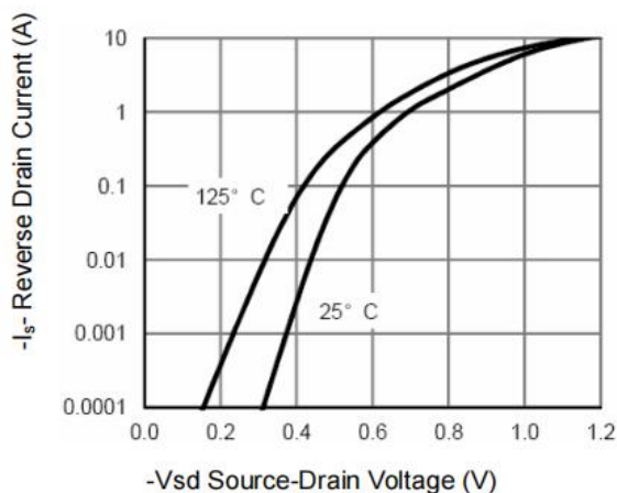
Figure 9: Diode Characteristics
