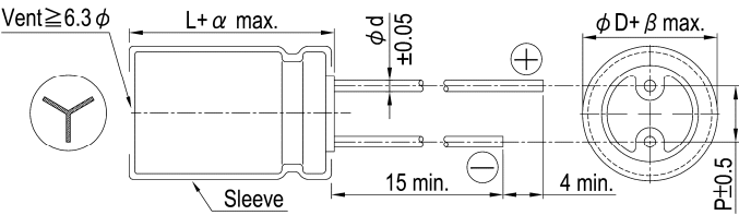
Lead Spacing & Diameter Unit: mm
