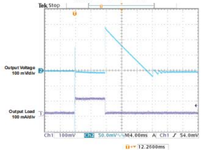
LOAD TRANSIENT RESPONSE VS TIME ( V_{\text{OUT}} = 5\text{ V} , C_L = 10\text{ }\mu\text{F} )
