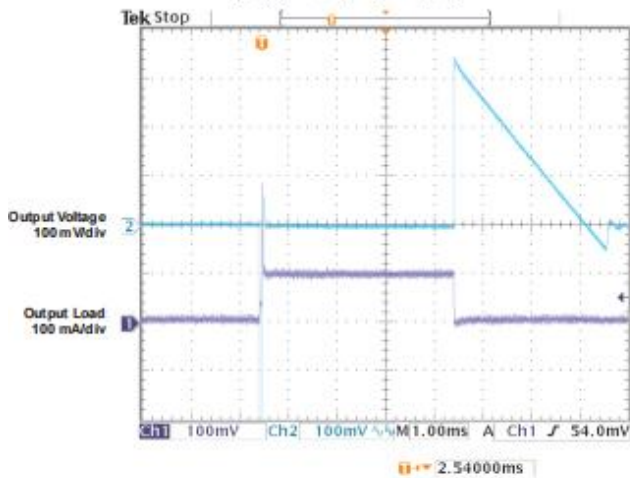
LOAD TRANSIENT RESPONSE VS TIME ( V_{\text{OUT}} = 5\text{ V} , C_L = 1\text{ }\mu\text{F} )
