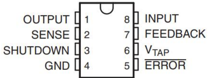
SOP-8
