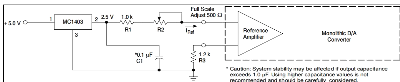
Figure 1. A Reference for Monolithic D/A Converters
