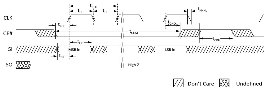
Figure 22: Input Timing
