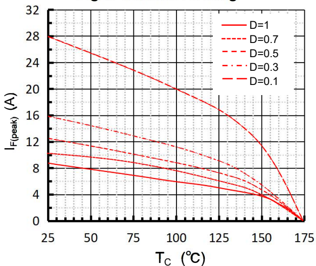
Fig 1. Current Derating
