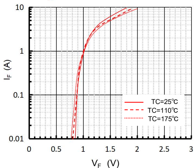
Fig 3. Forward Characteristics
