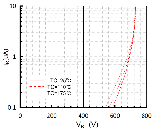
Fig 4. Reverse Characteristics
