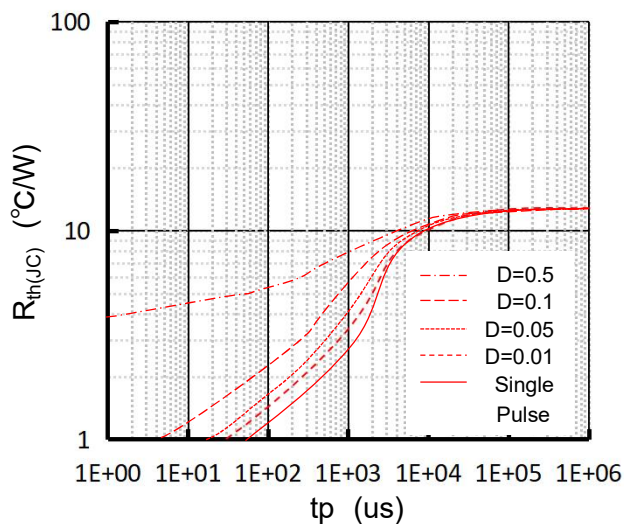
Fig 8. Transient Thermal Impandance
