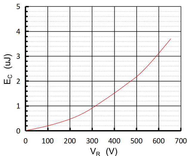
Fig 7. Typical Capacitance Stored Energy
