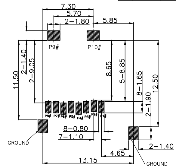
RECOMMENDED PCB LAYOUT (ALL TOLERANCE ARE ±0.05)
