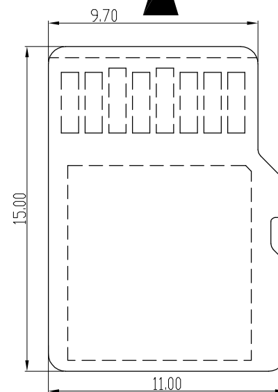
T-FLASH CARD
