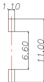
[P.C.B.LAYOUT]
