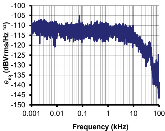
Figure 13: Typical noise voltage density e_{n0} with R_M = 50 \Omega
