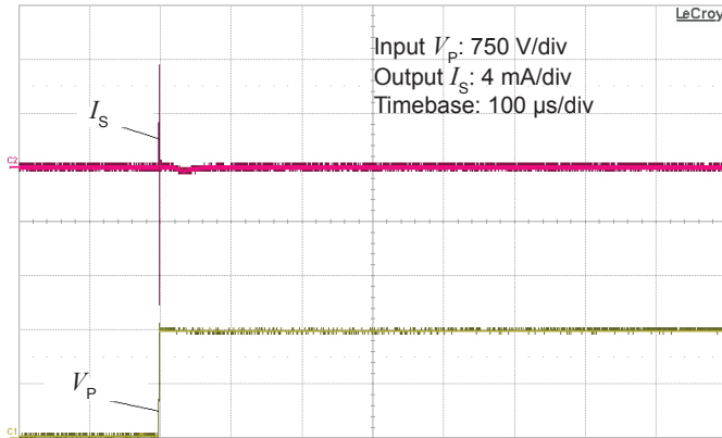
Figure 11: Typical common mode perturbation (1500 V step with 6 kV/μs R_M = 100 \Omega )
