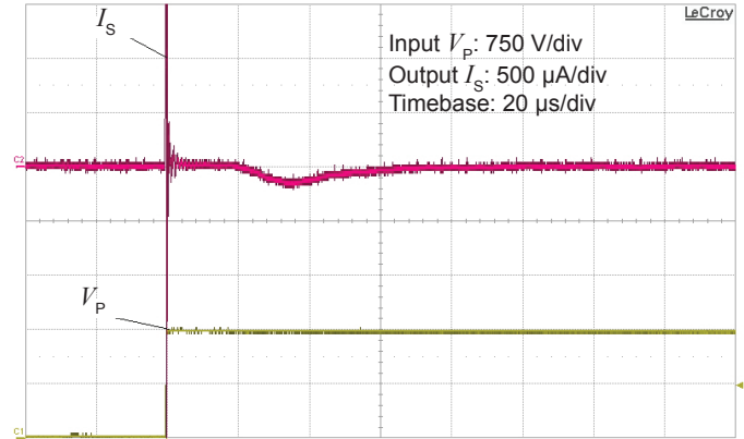
Figure 12: Detail of typical common mode perturbation (1500 V step with 6 kV/μs, R_M = 100 \Omega )
