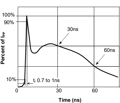
Fig.4 Pulse Waveform-ESD(IEC61000-4-2)
