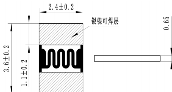
Overall dimension drawing (unit: mm)
