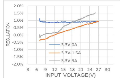
Line Regulation
