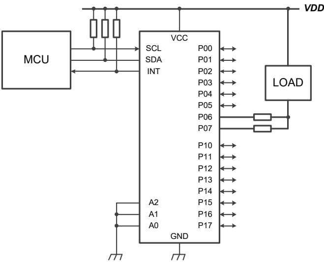
Figure 10. High Current-Drive Load Application
