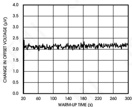
Figure 38. Warm-Up Time
