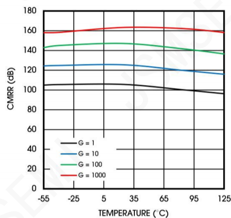
Figure 11. CMRR vs. Temperature
