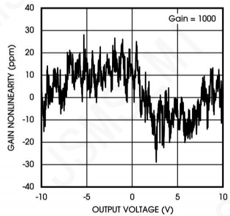
Figure 31. Gain Nonlinearity (G = 1000)
