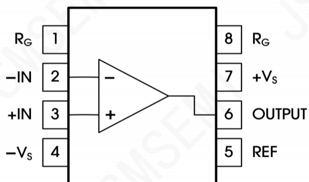
Figure 1. Pin Configuration
