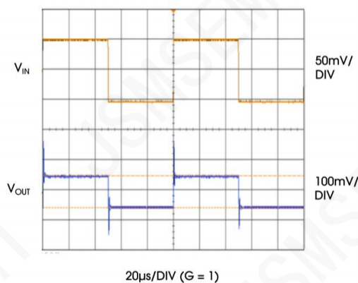
Figure 13. Small Signal Response (G = 1)
