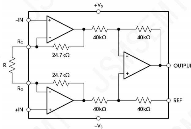
Figure 41. Functional Block Diagram
