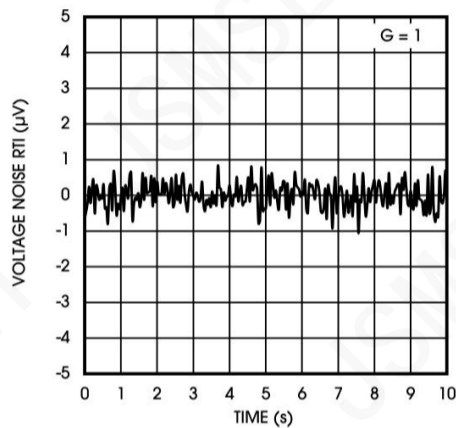
Figure 22. 0.1Hz to 10Hz RTI Voltage Noise
