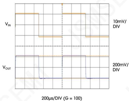
Figure 17. Small Signal Response ( G = 100 )
