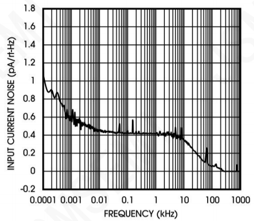
Figure 21. Input Current Noise Density
