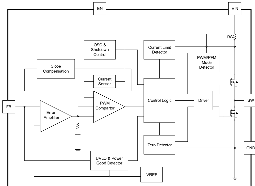
Block Diagram
