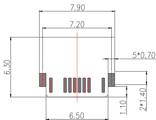
Cable Side PCB Layout (Tol:±0.05,T=0.80±0.05mm)
