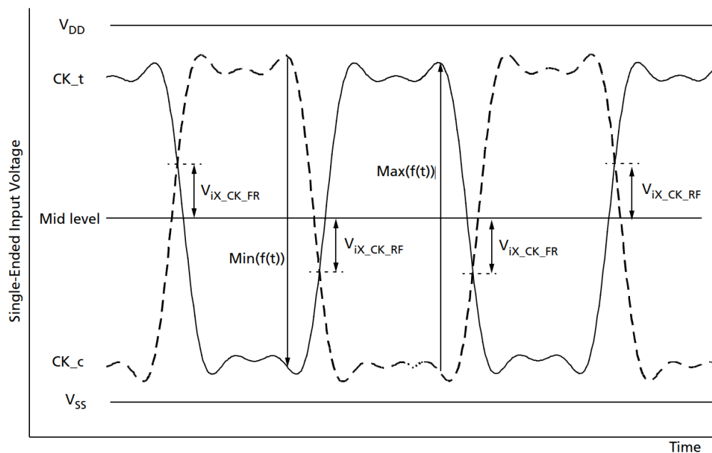
Figure — CK input cross-point voltage (Vix)
