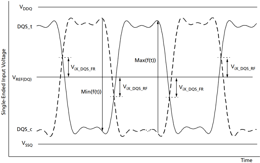
Figure — DQS input cross-point voltage (V)VIX Definition
