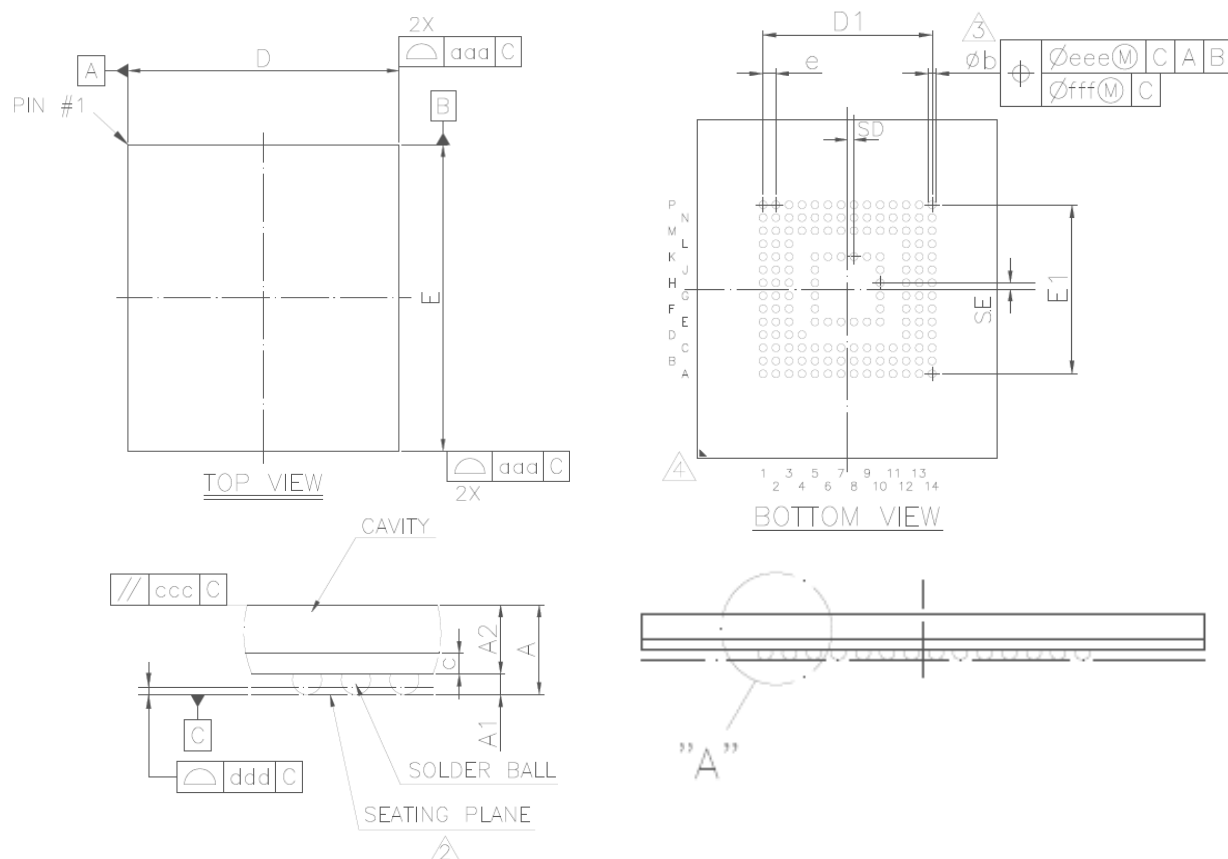
Figure 2 – Package Dimensions
