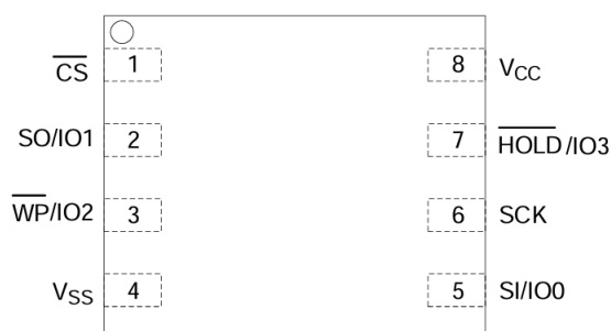
Figure 1. LGA8 Pin Assignment
