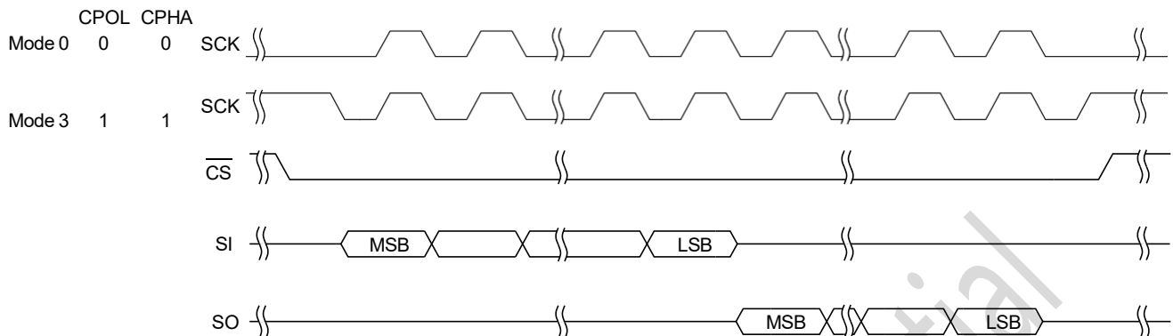
Figure 5. SPI Timing
