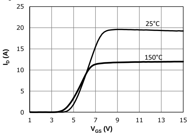
Fig 3: Transfer Characteristics
