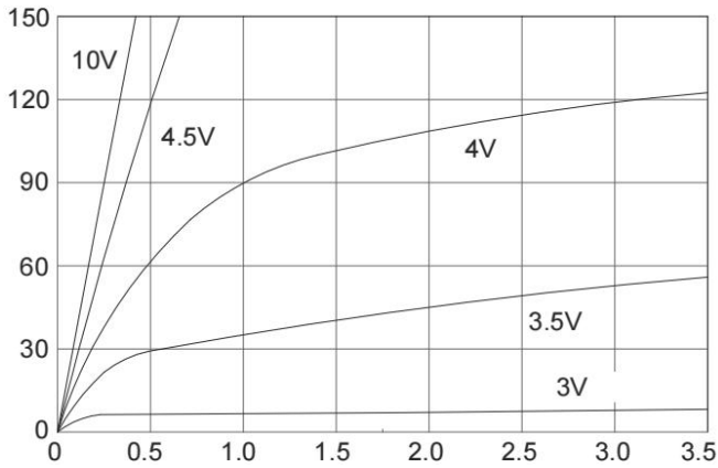
Figure 1: Output Characteristics
