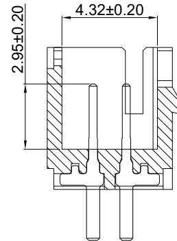
SECTION I-I
