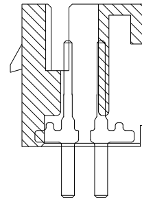
SECTION II-II
