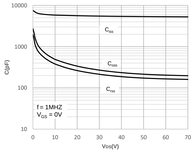
Figure 10: Capacitance Characteristics
