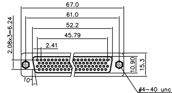
78 POSITION MALE/FEMALE
