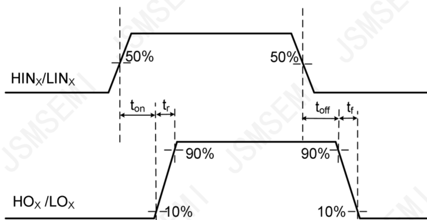
Figure 6-2 JSM6288 Input and output timing waveform
