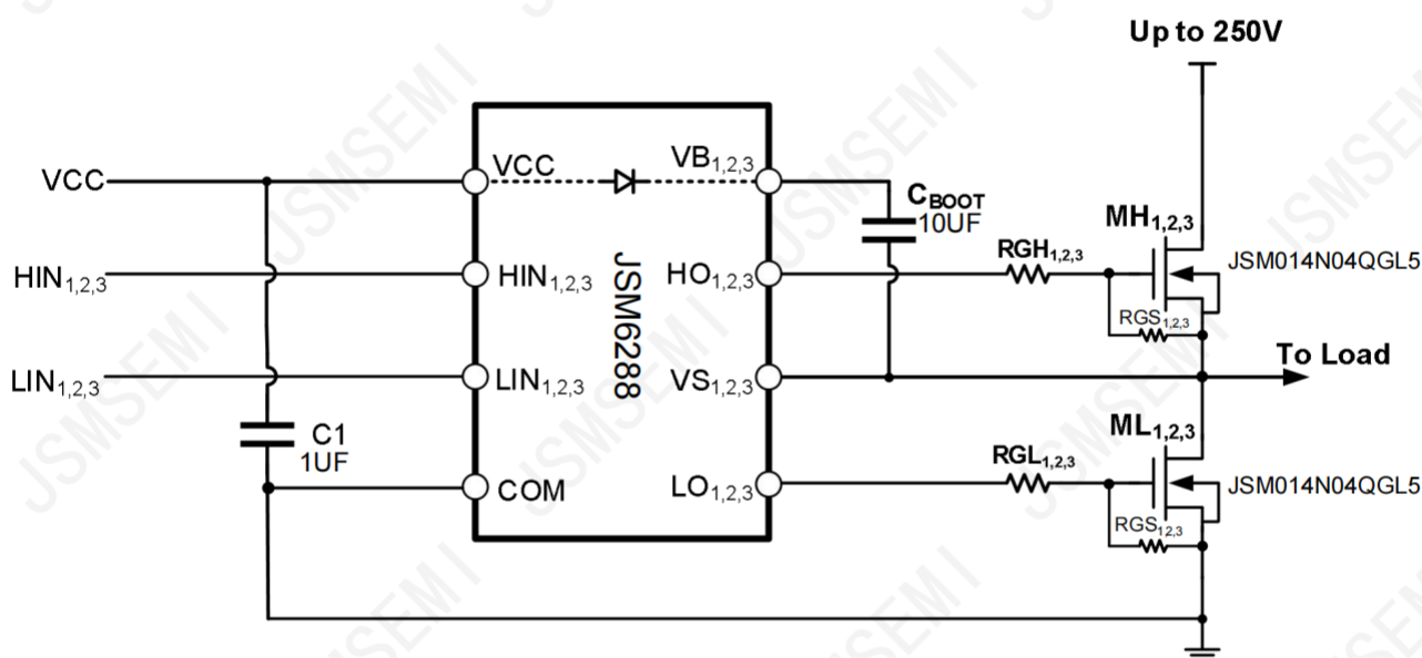
Figure 8-1 Typical application circuit of JSM6288
