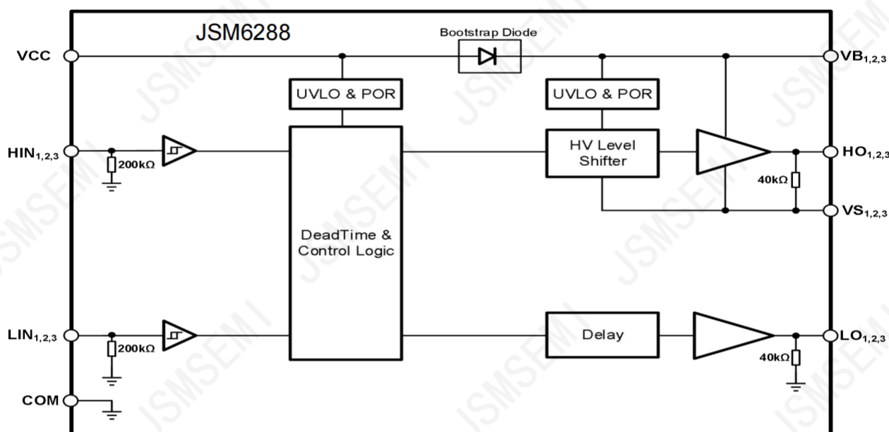
Figure7-1 Function Block Diagram of JSM6288
