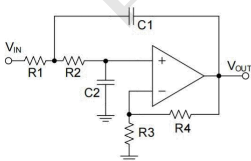
low-pass filter
