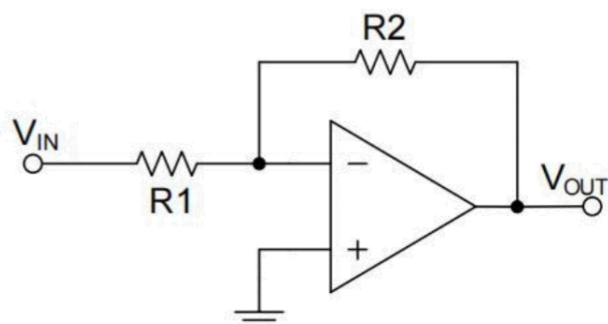
Reverse amplifier
