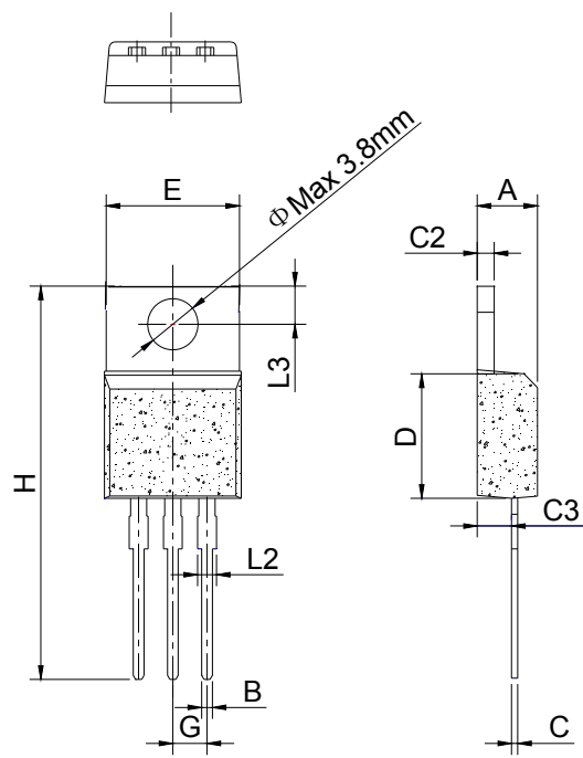
TO-220AB
