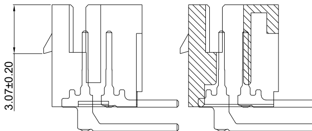
SECTION II-II
