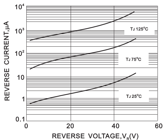
FIG. 2-TYPICAL REVERSE CHARACTERISTIC
