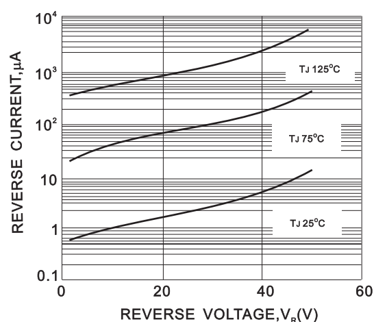
FIG. 2-TYPICAL REVERSE CHARACTERISTIC
