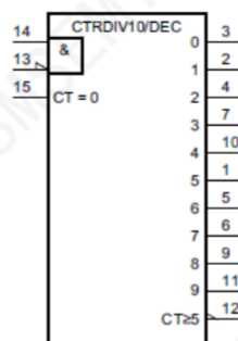
Figure 2. IEE logic symbol
