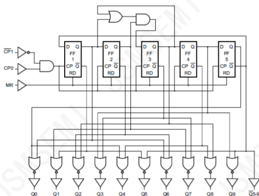
Figure 4. Logic diagram
