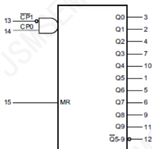
Figure 1. Logic symbol
