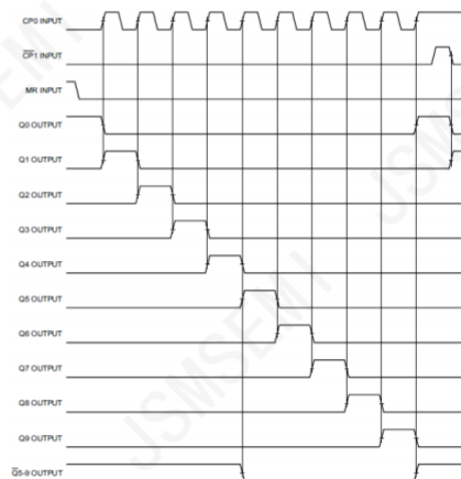
Figure 5. Timing diagram
