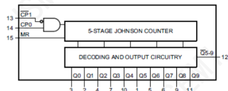
Figure 3. Functional diagram
