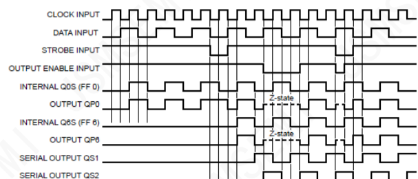
Figure 4. Timing diagram
