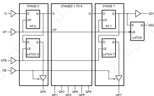
Figure 3. Logic diagram
