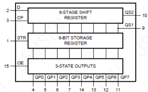
Figure 2. Functional diagram
