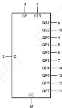
Figure 1. Logic symbol
