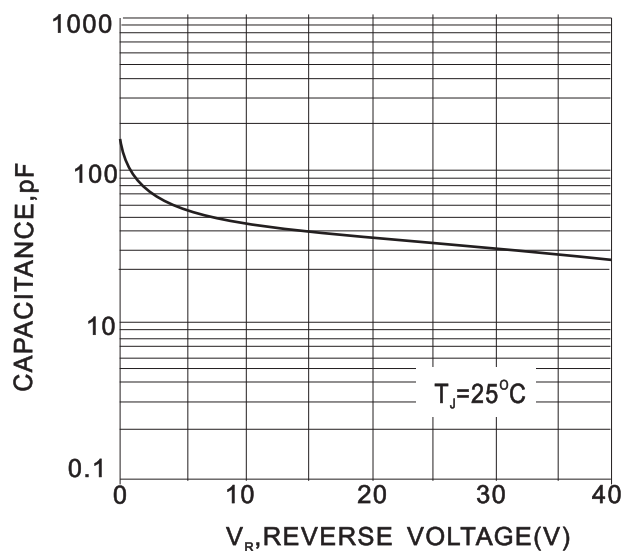
FIG. 3-TYPICAL JUNCTION CHATACTERISTIC
