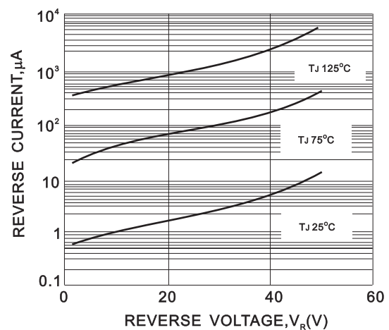
FIG. 2-TYPICAL REVERSE CHARACTERISTIC
