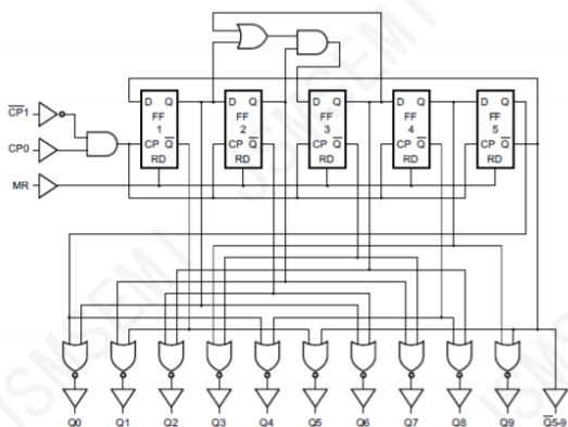
Figure 4. Logic diagram
