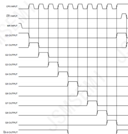
Figure 5. Timing diagram
