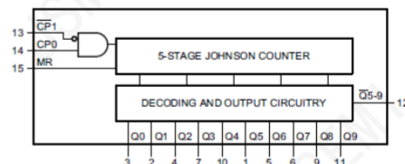
Figure 3. Functional diagram
