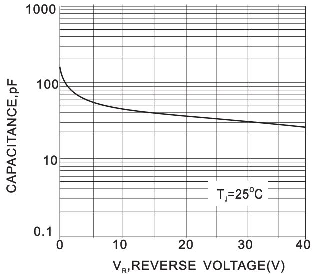
FIG. 3-TYPICAL JUNCTION CHATACTERISTIC
